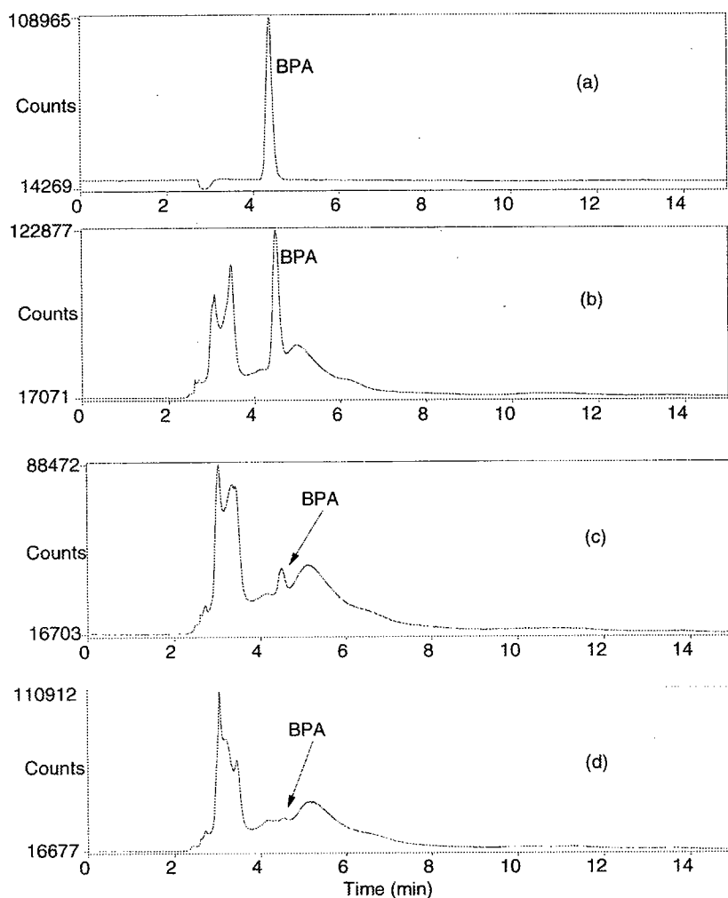
FIGURE 2 HPLC/Fluorescence Chromatograms of a) 99 ng BPA/mL Deionized water Standard. b) 99 ng BPA/mL Patrick's Bayou (PB) water. c) 13 ng BPA/mL PB water. d) 3 ng BPA/mL PB water
